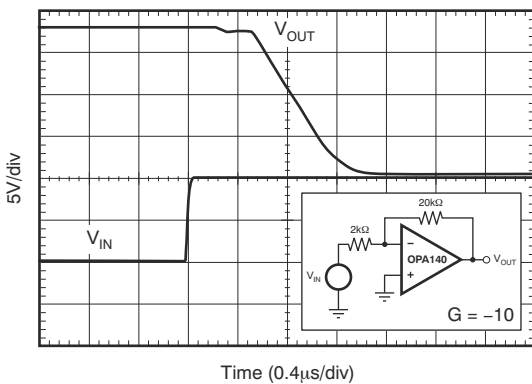
Figure 6-21. No Phase Reversal
