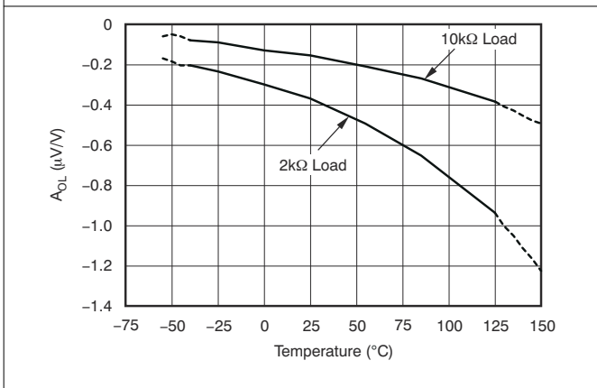
Figure 6-17. Open-Loop Gain vs Temperature
