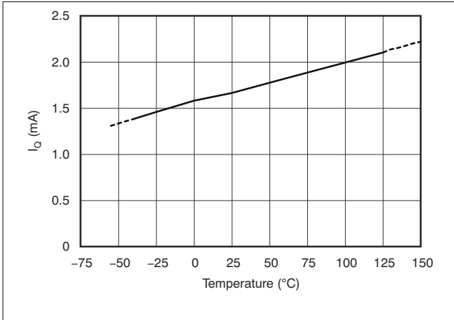
Figure 6-13. Quiescent Current vs Temperature
