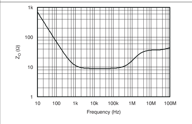
Figure 6-18. Open-Loop Output Impedance vs Frequency
