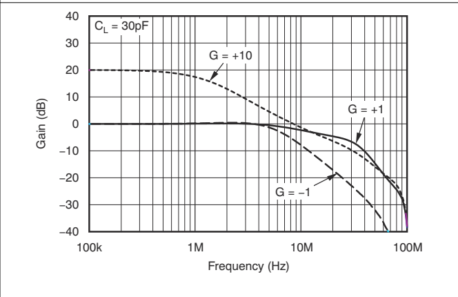
Figure 6-16. Closed-Loop Gain vs Frequency
