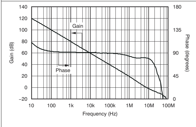
Figure 6-15. Gain and Phase vs Frequency
