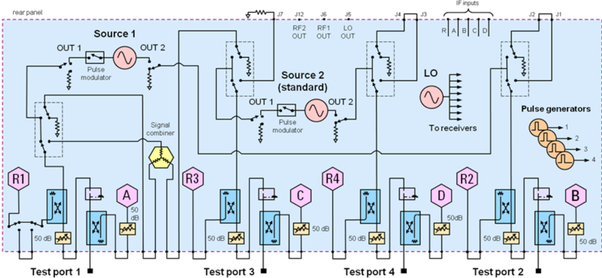
Figure 7. 4-Port N5247B Option 423
